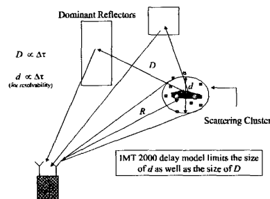
Figure 1: Geometry Assumed in Spatial Channel Model
