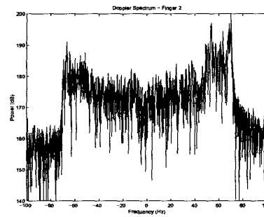
Figure 5: Doppler Spread for Urban Measurement Fingers 1 and 2 (speed = 25mph)
