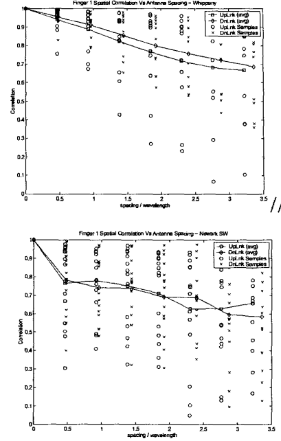
Figure 2: Scatter Plots of the Correlation Between Each Antenna and Antenna 1 for Suburban (top) and Urban (bottom) Environments on Uplink and Downlink Frequencies
