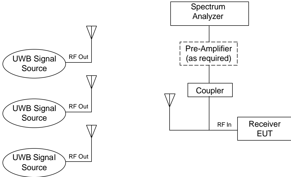
Figure7. Radiated Susceptibility Test Set-Up-Multiple Signal Method
