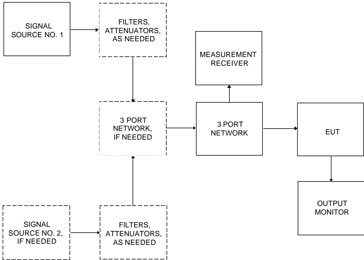
Figure 1. MIL-STD-461E CS104 General Test Setup.
