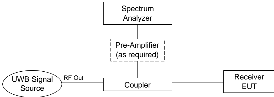
Figure 4. Setup for One Signal Susceptibility Test
