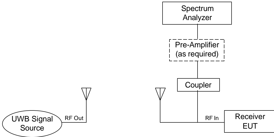
Figure 6. Radiated Susceptibility Test Set-Up-One Signal Method
