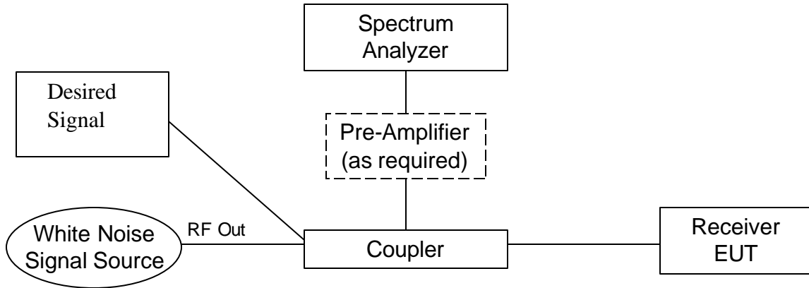
Figure 3. Setup for White noise Susceptibility Test
