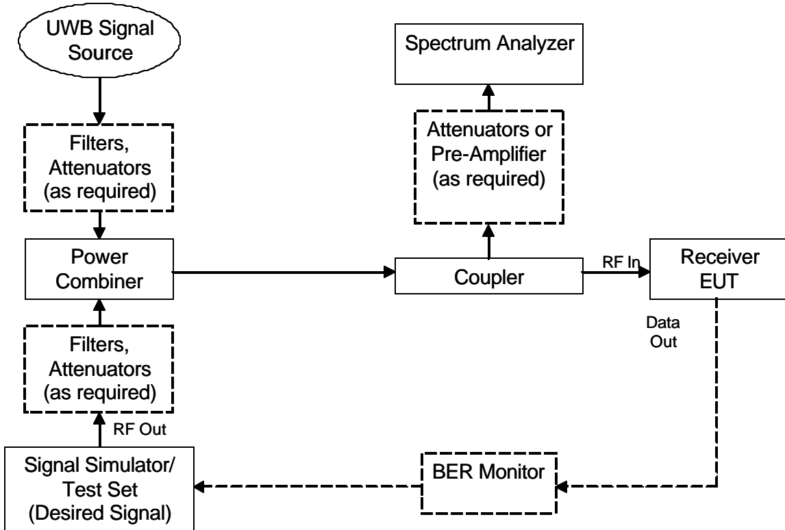
Figure 5. Setup for Two Signal Susceptibility Tests
