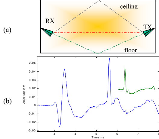
Figure 6: (a) Setup and (b) received waveform with both transmitter and receiver antennas pointing to the reflection surface.
