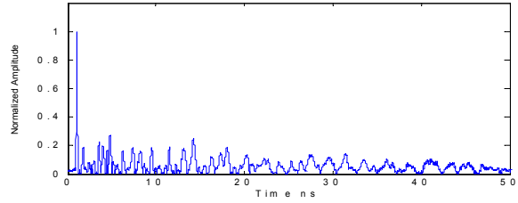
Figure 3. Typical line-of-site channel impulse response
