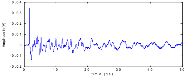
Figure 2. Typical received line-of-site multipath profile
